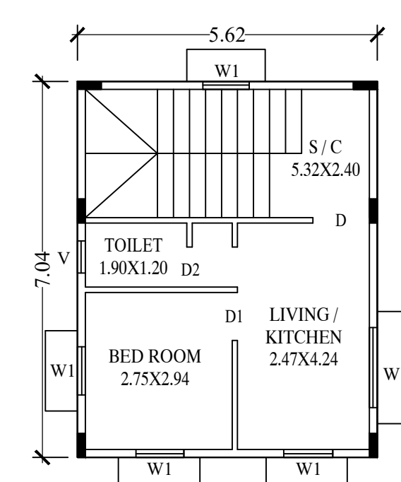
PROPOSED TYPICAL GROUND, FIRST & SECOND FLOOR PLAN
