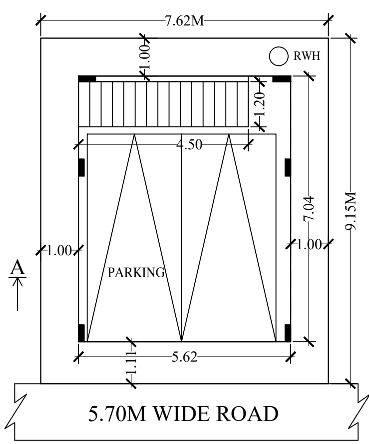
PROPOSED STILT FLOOR PLAN
